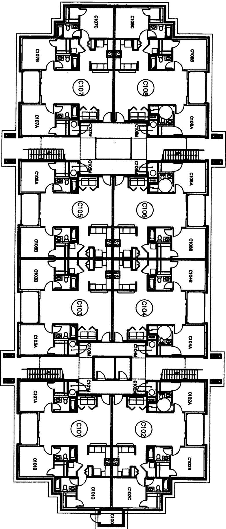
Building "C" - First Floor Plan NOT TO SCALE
