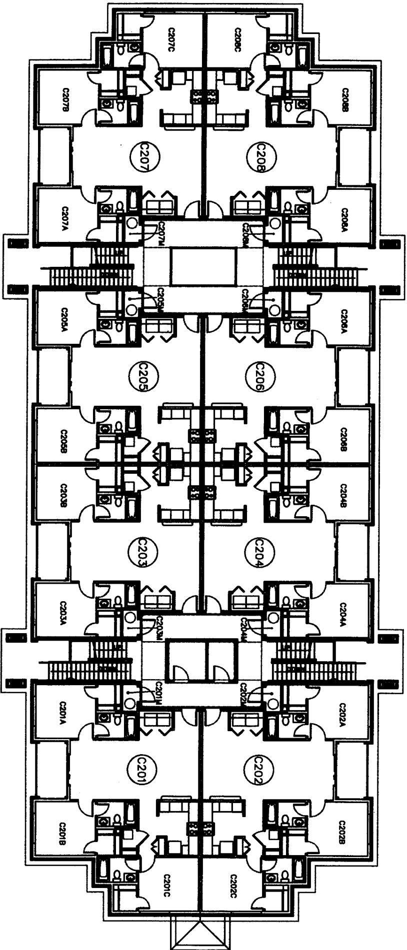
Building "C" - Second Floor Plan
